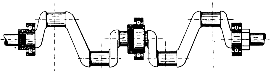
BALL-BEARING CRANKSHAFT ON NEW MERCEDES ENGINE AT PARIS SHOW.
